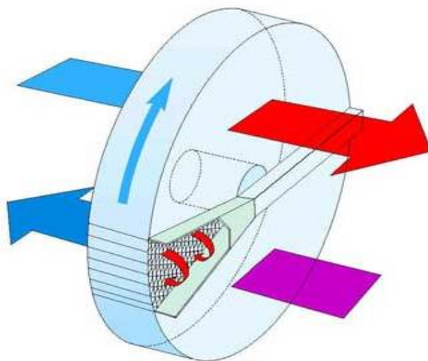
Fig. 3. Rotary recuperator
