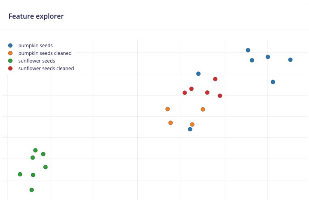
Fig. 4. Plot of all the data in dataset
