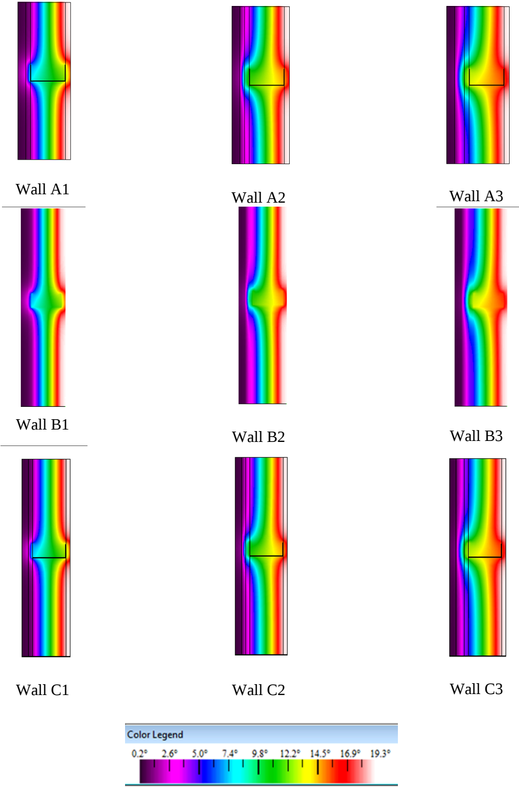
Fig. 2. Temperature profiles
